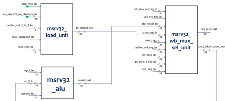
Pipeline Stage 3
